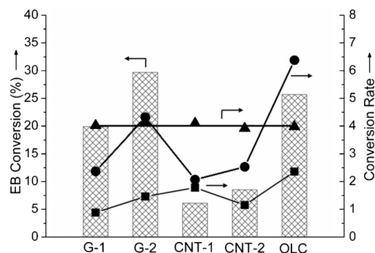
Figure 3. Comparisons of the ODH activity for various nanocarbon catalysts. EB conversion rate (bar) and conversion rates normalized by oxygen content (■; 10^{-7} molecules of EB converted per O atom per second), surface area (●; 10^{-4} molecules of EB converted per \text{nm}^2 per second) and number of active sites (TOF; ▲; 10^{-4} molecules of EB converted per ketonic carbonyl group per second), respectively. Conditions: 538 K, 2.8 kPa EB, 1.4 kPa \text{O}_2 , balance He, 100 mg catalyst.
