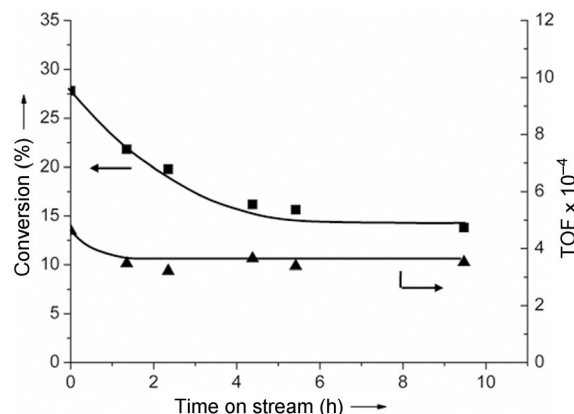
Figure 4. EB conversion (■) and TOF value (▲) for the OLC catalyst as a function of time on stream. TOF value is given as molecules of EB converted per carbonyl group per second. Conditions: 538 K, 2.8 kPa EB, 1.4 kPa \text{O}_2 , balance He, 100 mg OLC catalyst.
